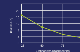
Battery Mode
