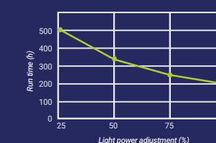
Hybrid Mode
